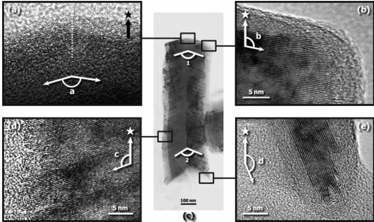
Figure 3. Lattice images a of single carbon fragment: a) a convex end exhibits the mirror symmetry of both sets of graphenes planes. b) Lattice image of an edge. c) TEM image of a fragment. d) Image of a shoulder. e) Image of the concave end. The arrow with a star indicates the direction of the fiber axis.
