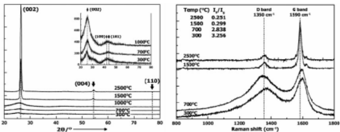
Figure 1. a) X-ray diffraction pattern and b) Raman spectrum for thermally treated samples. The inset in figure 1a is an expanded plot showing fibers related to different pyrolysis temperatures.
